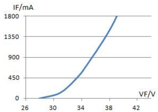
4、Voltage Vs Current
